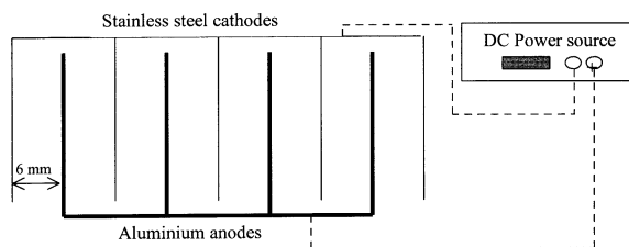
Fig. 4. Schematic diagram of electrode arrangement.
