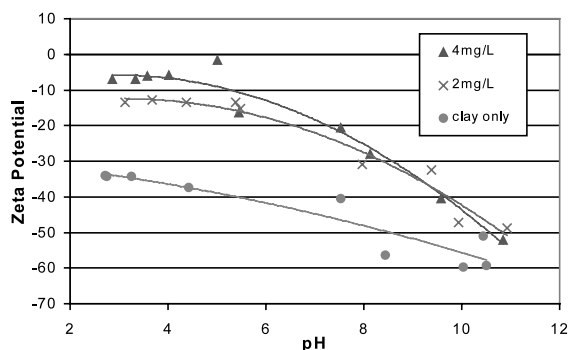
Fig. 7. Zeta potential for 1 g l -1 clay solutions subjected to chemical dosing at 0, 2 and 4 mg-Al l -1 of alum.
