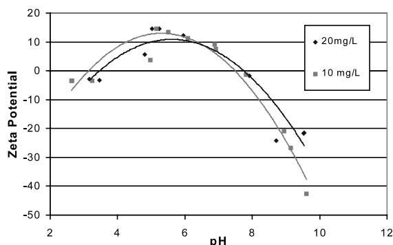
Fig. 8. Zeta potential for 1 g l -1 clay solution subjected to chemical dosing at 10 and 20 mg-Al l -1 of alum.
